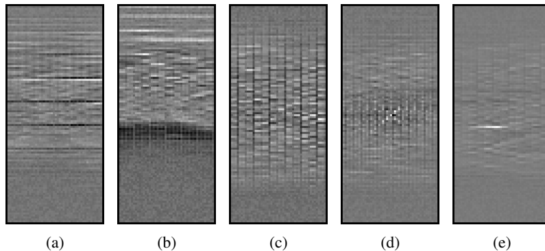
Figure 3: Some hand-selected features from \mathbf{L}_1 that are representative for the types of patterns learned from the note-centered representation (see Figure 2b). Dark values correspond to negative weights, light values to positive weights.
